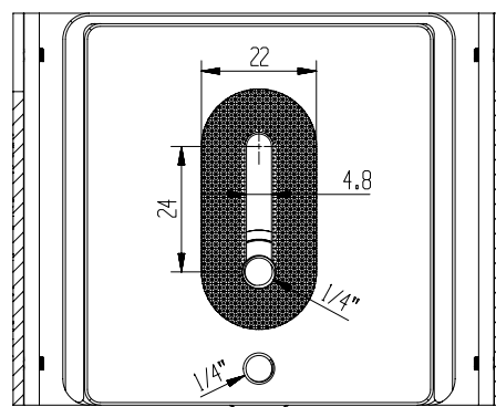
Mounting Plate
